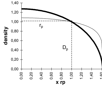
Fig.38. Density and energy of ec's versus proton radius
